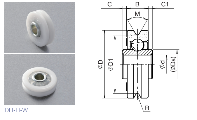
Model 2 Inner ring (Inner race width: Wide)
