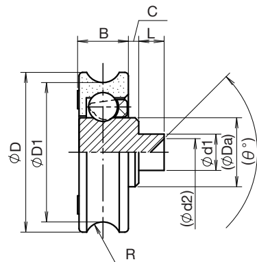
Riveting shaft
