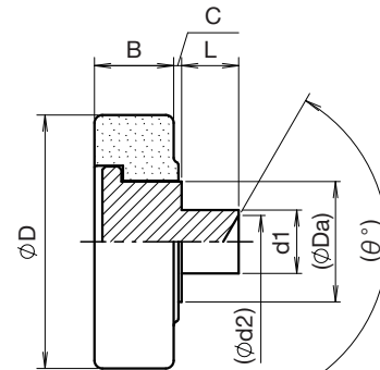
Model 2 Riveting shaft
