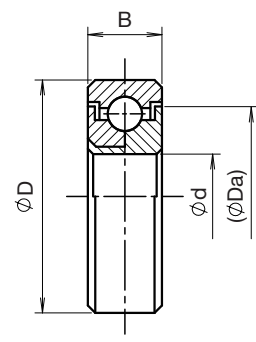
Model 2 Inner ring (Full ball)
