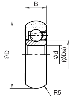
Inner ring
