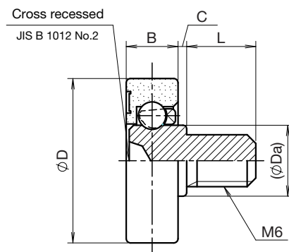
Model 1 Screw shaft (Cross recessed head)
