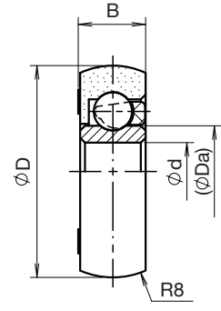
Inner ring (R8 type)
