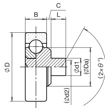
Model 1 Riveting shaft (Full ball)
