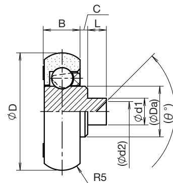
Riveting shaft
