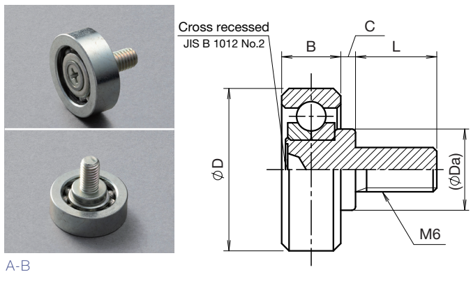
Model 3 Screw shaft (Cross recessed head and full ball)
