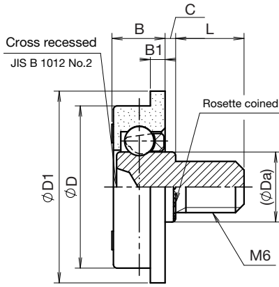
Model 2 Screw shaft (Cross recessed head and rosette coined)
