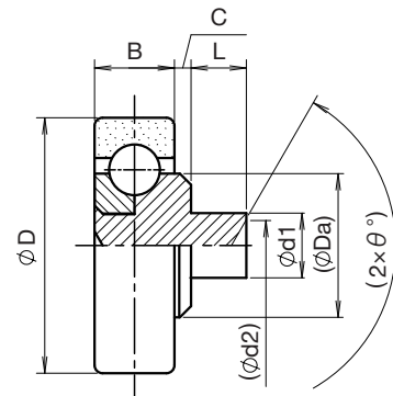
Model 1 Riveting shaft (Full ball)
