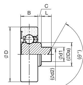
Model 2 Riveting shaft (Retainer)
